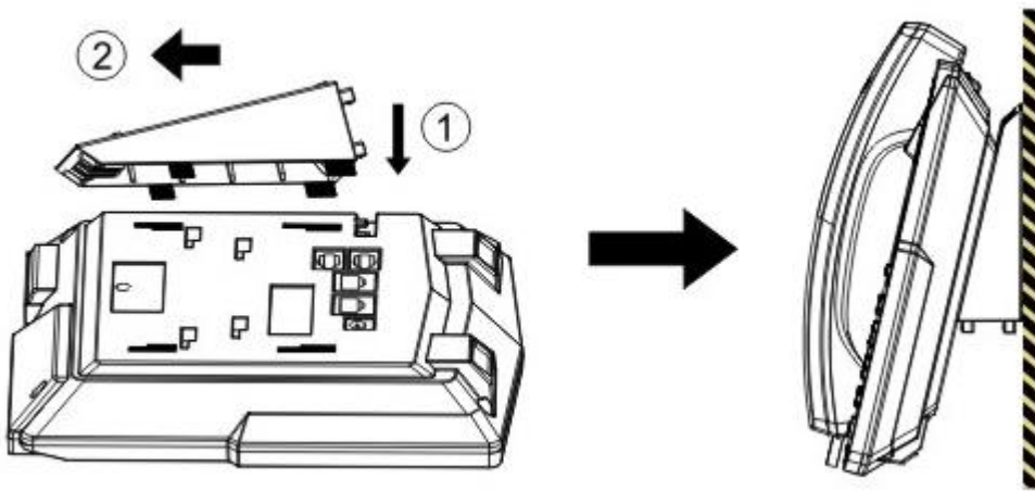
Figure 2 - Wall-mount Installation
